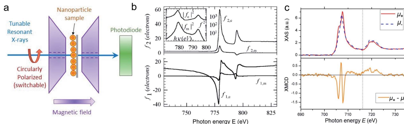
Fig. 9 XAS and XMCD measurements on MNPs. (a) Sketch of the experimental setup showing the MNP film placed in transmission geometry under an out-of-plane in situ magnetic field and transmitted light detected downstream on a photodiode. (b) XAS data collected on 9 nm Co MNPs, displaying the real ( f_1 ) and imaginary ( f_2 ) parts of the charge ( f_c ) and magnetic ( f_m ) atomic scattering factors. Reprinted figure with permission from Kortright et al. 278 Copyright 2005 by the American Physical Society. (c) XAS (top) and associated XMCD (bottom) data collect on 8 nm \text{Fe}_3\text{O}_4 MNPs. Adapted from Cai et al. 279 Rights managed by AIP Publishing.
