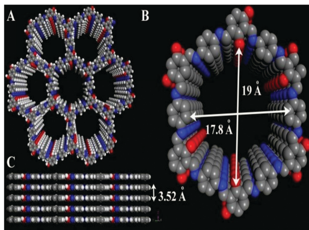
Fig. 3 The 3D structure of \text{Ag@COF} . Reproduced with permission from ref. 21; copyright: 2019, Chemistry An Asian Journal.
