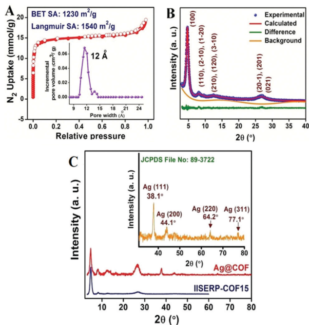
Fig. 4 (A) The \text{N}_2 adsorption isotherm of IISERP-COF-15. (B) The PXRD pattern of the COF. (C) The PXRD pattern of \text{Ag@COF} . Reproduced with permission from ref. 21; copyright: 2019, Chemistry An Asian Journal.
