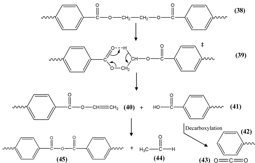
Scheme 5 Fundamental reactions for the thermal decomposition of PET. The symbol \ddagger indicates a transition state. Arabic numerals indicate chemical species and intermediates formed during the pyrolysis of PET.
