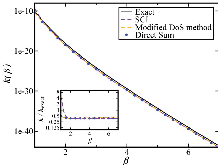
Fig. 3 A comparison of the exact thermal rate, the semiclassical instanton rate (eqn (26)) and the thermalised microcanonical rates from the direct-sum method (eqn (68)) and the modified DoS method (eqn (88)), for model 1, with V_{\text{TS}} = 20 , a_{\text{eck}} = 1 , a_{\omega} = 1 , \omega_{\text{TS}} = 5 and \omega_r = 20 . The inset shows the relative error.
