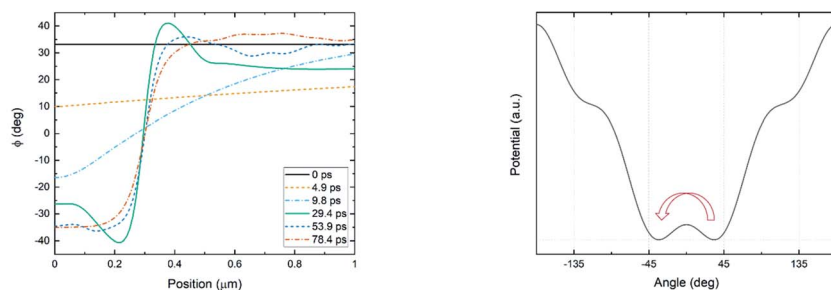
Fig. 3 (a) Snapshots of the spin deflection angle in the strongly nonlinear regime, when the bias magnetic field is applied along the x -axis. After forming the domain wall between the initial and the switched orientations, the various modes of the spin wave are emitted from the wall. (b) The potential landscape set by the bias field with the two stable states. The THz excitation enabled the spin around the antenna to flip to the alternative stable state.
