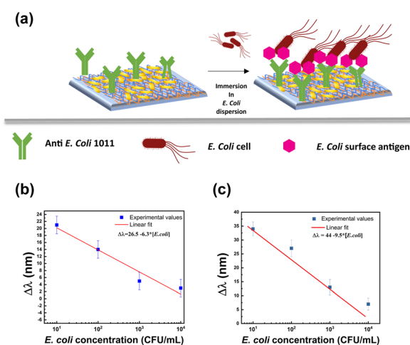
Fig. 7 Schematic of the mechanism of capturing E. coli cells promoted by the Ab incorporated on the plasmonic substrate. (a) Optical shift ( \Delta\lambda ) as a function of E. coli concentration in the incubation dispersion, reported on a logarithmic scale for E. coli recognition experiments in the presence of SYTO 9 TM (b) and in the absence of SYTO 9 TM (c).
