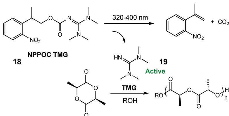
Scheme 12 A photocaged tetramethyl guanidine which releases the active species TMG for ROP of \epsilon -LA. 79 Reproduced from ref. 79 with permission from the Royal Society of Chemistry.
