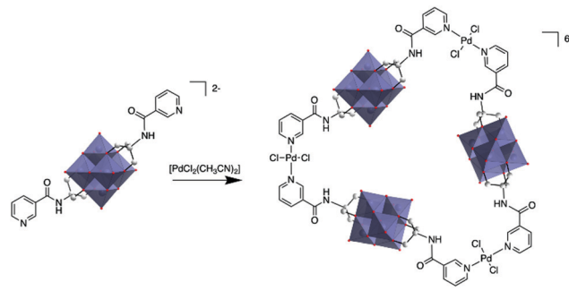
Fig. 4 Synthesis of a POM-based trimer from a bis(pyridine-trisalkoxo)-hexavanadate anion and trans - [\text{PdCl}_2(\text{CH}_3\text{CN})_2] . This figure has been adapted from ref. 80 with permission from the Royal Society of Chemistry, copyright 2012.
