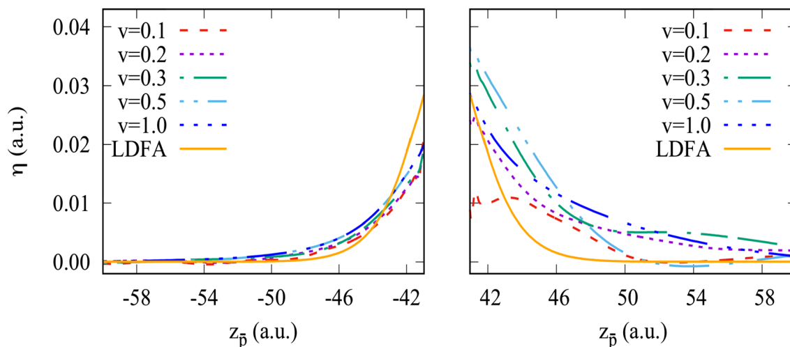
Fig. 8 The same as Fig. 7 but for the Na 1074 cluster.
