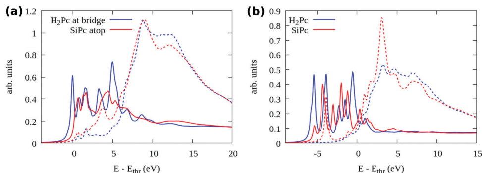
Fig. 9 Comparison of the simulated N 1s NEXAFS between (a) bridge \text{H}_2\text{Pc}/6\text{H-SiC}(0001)-(3 \times 3) and top \text{SiPc}/6\text{H-SiC}(0001)-(3 \times 3) , (b) gas phase \text{H}_2\text{Pc} and \text{SiPc} . The solid lines represent photon polarization along the surface normal and the dotted ones in the surface plane.
