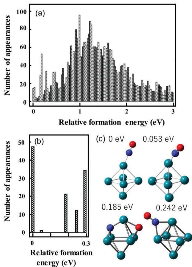
Fig. 3 Histograms of relative energies of \text{Rh}_6^+(\text{NO}) isomers calculated at the B3LYP/LANL2DZ (a) and B3LYP/sdd (b) levels of theory. For (b) all geometries in the [0,0.5 eV] interval in (a) were reoptimized. (c) Geometries of the four lowest-energy isomers in (b). Panel (a) reprinted with permission from ref. 97. Copyright (2021) Elsevier.
