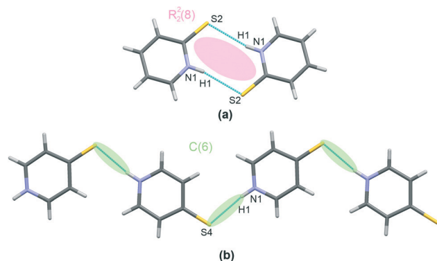
Fig. 3 I–IV characteristic patterns of the self-assembly of mercaptopyrindines via hydrogen bonding. The R_2^2(8) dimer present in II and IV – (a), and the C(6) chain in III – (b). Atoms are marked with colours, as follows: N – blue, S – yellow, C – grey, and H – white. The classification of synthons according to graph set method is also given.
