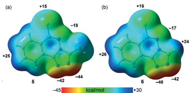
Fig. 9 MEP surfaces (isosurface 0.001 a.u.) of 5 (a) and 6 (b) at the PBE0-D3/def2-TZVP level of theory. The MEP values at selected points of the surfaces are given in \text{kcal mol}^{-1} .
