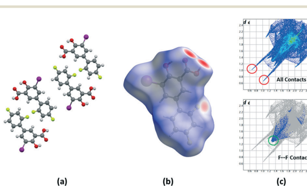
Fig. 3 (a) Unit cell representation of the IDIF_ Anti domain, (b) Hirshfeld surface mapped with d_{norm} and (c) fingerprint plots computed from Hirshfeld surfaces. Strong H...O contacts are highlighted in red and F...F contacts in green.
