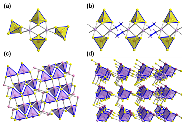
Fig. 5 Molecular structure of the [Mn_2As_4S_{16}]^{8-} cluster anion (a), fragment of the 1D- \{[Mn_2As_2S_8](N_2H_4)_2]\} strand formed from \mu -N 2 H 4 -linked [Mn_2As_2S_8]^{6-} clusters (b), view of the 2D- \{[Cu_3As_2S_5]^{-}\} layer (c) and the open-framework constructed by [MnAs_3S_6]^{-} clusters (d). Counterions are omitted for clarity. Color code: As-plum, Mn-lavender, Cu-rose, S-yellow, N-blue.
