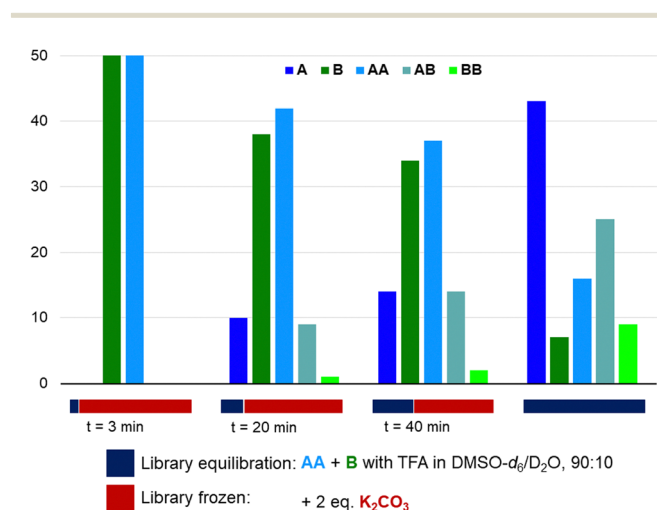
Fig. 4 The equilibration of a library starting from AA (14 mM) and B (14 mM) with TFA (14 mM) in DMSO-d 6 /D 2 O (90:10) can be brought to a halt by the addition of K 2 CO 3 (28 mM). The libraries were analysed by 1 H NMR spectroscopy after 5 hours, independent of the moment at which the library was frozen, and the results are shown in mol%.
