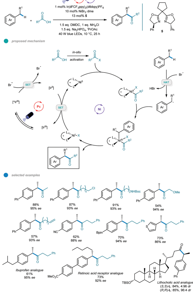
Scheme 11 Photoredox and nickel dual-catalyzed asymmetric acylations of benzylic C–H bonds with carboxylic acids.
