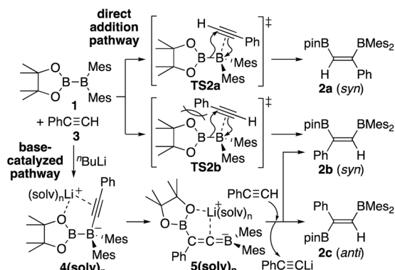
Scheme 3 Proposed mechanism for direct and base-catalyzed diboration of phenylacetylene by using pinB-BMes 2 .
