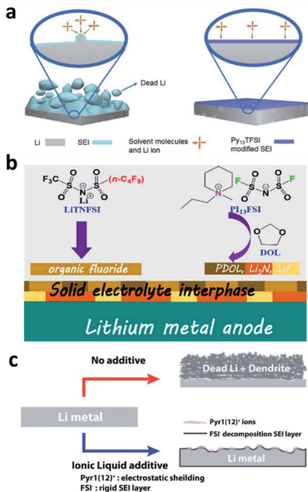
Fig. 10 The use of an ionic liquid in the electrolyte for forming nitrated interfaces on Li metal electrodes. (a) Schematic illustration of the use of the \text{Py}_{13}\text{TFSI} ionic liquid in an ether electrolyte for stabilizing the Li metal electrode; 100 reproduced with permission. Copyright 2017, John Wiley and Sons. (b) Illustration of the co-use of the \text{PL}_{13}\text{FSI} ionic liquid and \text{LiTFSI} to construct a nitrated composite SEI on the Li metal electrode; 101 reproduced with permission. Copyright 2018, American Chemical Society. (c) Illustration of the application of \text{Pyr1(12)FSI} to regulate the uniform deposition of \text{Li}^+ and reduce dead Li. 102 Reproduced with permission. Copyright 2018, John Wiley and Sons.
