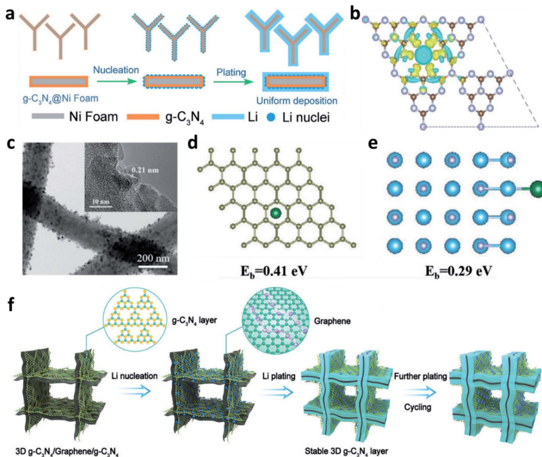
Fig. 13 (a) Schematic illustration of the preparation of a g-C 3 N 4 layer on Ni foam and its effects towards regulating Li + uniform deposition; (b) charge distribution of the g-C 3 N 4 layer revealing that N atoms have higher electron density and can absorb positively charged Li + ; 134 reproduced with permission. Copyright 2019, John Wiley and Sons. (c) TEM images of the TiN-decorated 3D carbon fibre; (d) optimized geometries for calculating the binding energy of a Li atom adsorbed on TiN, and (e) the corresponding charge density difference; 136 reproduced with permission. Copyright 2019, John Wiley and Sons. (f) Schematic illustration of the Li deposition on the 3D g-C 3 N 4 /G/g-C 3 N 4 electrode. 137 Reproduced with permission. Copyright 2021, John Wiley and Sons.
