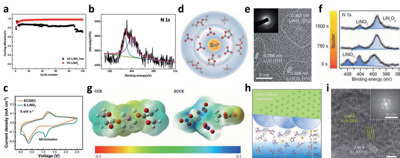
Fig. 7 The use of the \text{LiNO}_3 additive in carbonate-based electrolytes. (a) CE of a Li-Cu cell in a carbonate electrolyte with and without VC- \text{LiNO}_3 as the additive and (b) N 1s XPS spectrum of the cycled Li; 90 reproduced with permission. Copyright 2015, Elsevier. (c) Cyclic voltammetry (CV) curves of Li-Cu cells with and without \text{CuF}_2 - \text{LiNO}_3 co-additives, where an additional peak belonging to \text{LiNO}_3 decomposition at \sim 1.1 V can be observed; 91 reproduced with permission. Copyright 2018, John Wiley and Sons. (d) Structural illustration of the \text{Sn}^{2+} solvated sheath; (e) high resolution TEM (HRTEM) image of the SEI formed in the carbonate electrolyte with \text{Sn}(\text{OTf})_2 - \text{LiNO}_3 additives, with the corresponding selected area electron diffraction pattern in the inset; (f) N 1s XPS depth profiles for the SEI formed in the electrolyte with \text{Sn}(\text{OTf})_2 - \text{LiNO}_3 additives; 35 reproduced with permission. Copyright 2020, John Wiley and Sons. (g) Electrostatic potential (ESP) images for the solvated EC and DEC molecules in the electrolyte with and without \text{In}(\text{OTf})_3 - \text{LiNO}_3 as an additive; (h) schematic illustration of the formation of an inorganic wavy SEI; (i) cryo-TEM image of the inorganic wavy SEI showing the presence of \text{Li}_3\text{N} . 92 Reproduced with permission. Copyright 2020, John Wiley and Sons.
