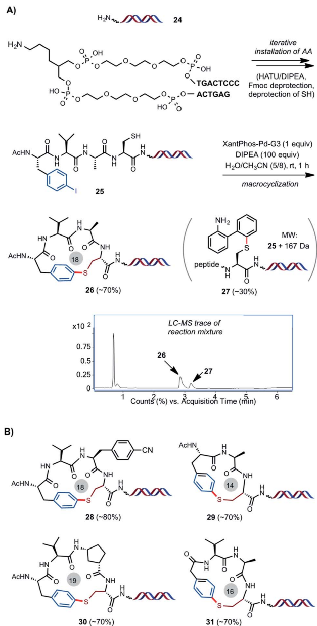
Scheme 4 (A) Construction of S-aryl ether-linked peptide macrocycle on uncoded DNA template. (B) Representative model synthesis on DNA. The side products sometimes overlap with the desired cyclized product on LC. Yields/conversion were based on the estimation of MS signals of the corresponding peaks on LC.
