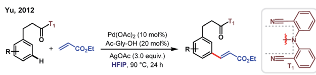
Scheme 5 First instance of Pd(II)-catalyzed meta-C(sp²)-H olefination of hydrocinnamic acids in HFIP medium.
