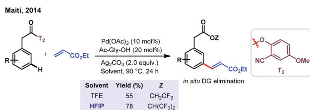
Scheme 6 Remarkable solvent effect by HFIP in Pd(II)-catalyzed meta-C(sp²)-H olefination of aryl acetic acids.
