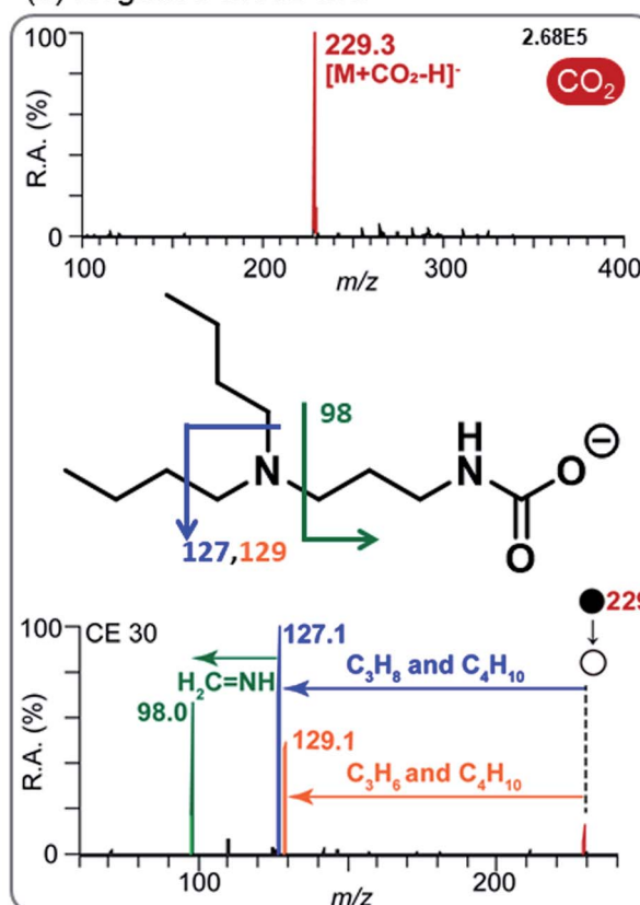
Fig. 1 DBPA/CO 2 droplet reaction by adding CO 2 in the gas phase (a) Droplet reaction of amine/CO 2 conducted by ESSI. (b) Positive and (c) negative mode mass spectra and MS/MS spectra showing fragmentation of protonated and deprotonated DBPA carbamic acid.
