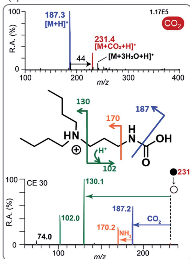
Fig. 1 DBPA/CO 2 droplet reaction by adding CO 2 in the gas phase (a) Droplet reaction of amine/CO 2 conducted by ESSI. (b) Positive and (c) negative mode mass spectra and MS/MS spectra showing fragmentation of protonated and deprotonated DBPA carbamic acid.
