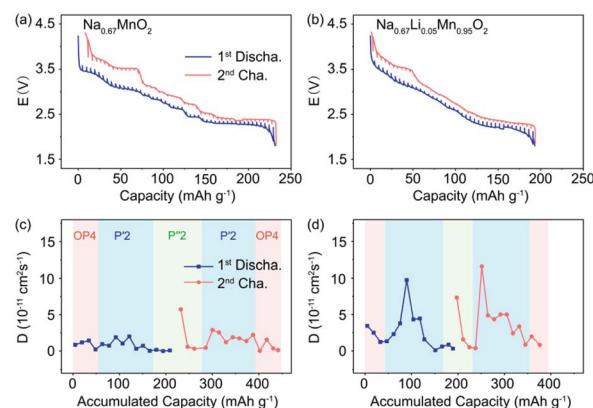
Fig. 5 GITT profiles of (a) \text{P}'2\text{-Na}_{0.67}\text{MnO}_2 and (b) \text{P}'2\text{-Na}_{0.67}\text{Li}_{0.05}\text{Mn}_{0.95}\text{O}_2 in a charge and discharge cycle. \text{Na}^+ diffusion coefficients of (c) \text{P}'2\text{-Na}_{0.67}\text{MnO}_2 and (d) \text{P}'2\text{-Na}_{0.67}\text{Li}_{0.05}\text{Mn}_{0.95}\text{O}_2 calculated from GITT measurements.
