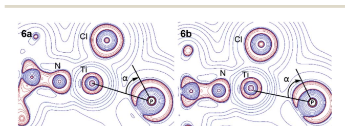
Fig. 8 Contour map of \nabla^2\rho in the \text{P}_\text{C} –Ti–Cl plane for 6a and 6b (red lines indicate charge concentration and blue lines indicate charge depletion).
