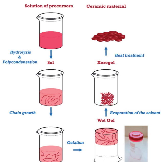
Fig. 5 Diagram illustration the sol–gel process. This figure has been reproduced from ref. 82 with permission from MDPI, copyright 2019.
