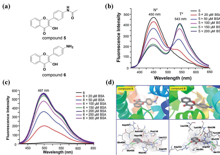
Fig. 9 (a) The structure of compound 5 and 6 ; (b, c) fluorescence spectra of 20 μM compound 5 (b) and 6 (c) upon addition of different concentrations of BSA in 50 mM Tris-buffer (pH 7.4). Excitation wavelength for compound 5 = 365 nm. Excitation wavelength for compound 6 = 395 nm; (d) the interactions between compound 5 and 6 and BSA visualized by molecular docking simulations. 100
