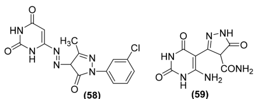
Fig. 14 Chemical structures of pyrazolediazenylpyrimidine derivative (58) and pyrazolone derivative (59).
