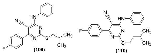
Fig. 31 Chemical structures of selected 6-(4-fluorophenyl)-pyrimidine-5-carbonitrile derivatives (109 and 110).
