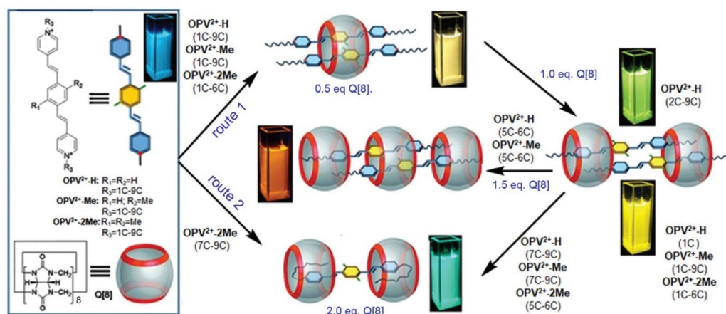
Scheme 1 Chemical structures of \text{OPV}^{2+} derivatives and \text{Q}[8] , and representation of \text{Q}[8] -based dynamic host-guest assemblies with multiple tunable fluorescence signals. Route 1: \text{Q}[8] concentration dependent host-guest interactions of 2 : 1, 2 : 2, 2 : 3, and 1 : 2 (guest/ \text{Q}[8] ); route 2: the formation of a U-shaped conformation of \text{Q}[8] with \text{OPV}^{2+}\text{-2Me} (7C-9C).
