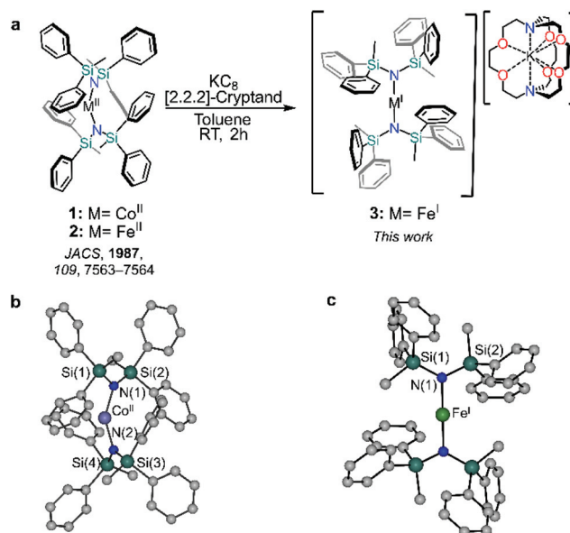
Fig. 1 Preparation of 1–3 and single crystal X-ray structure determinations of 1 and 3 . (a) Reaction scheme for the synthesis of [\text{M}\{\text{N}(\text{SiMePh}_2)_2\}_2] ( 1 , \text{M} = \text{Co}^{\text{II}} ; 2 , \text{M} = \text{Fe}^{\text{II}} ) and [\text{K}(2,2,2\text{-crypt})][\text{Fe}\{\text{N}(\text{SiMePh}_2)_2\}_2] ( 3 , \text{M} = \text{Fe}^{\text{I}} ). Solid-state molecular structures of 1 (b) and 3 (c) H atoms and [\text{K}(2,2,2\text{-cryptand})]^+ were omitted for clarity.
