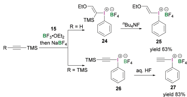
Scheme 10 Access to \alpha -silyl substituted (E) -configured vinylidonium salt 24 and subsequent stereoretentive protodesilylation to give 25 and synthesis of ethynyl(phenyl)iodonium tetrafluoroborate (27).
