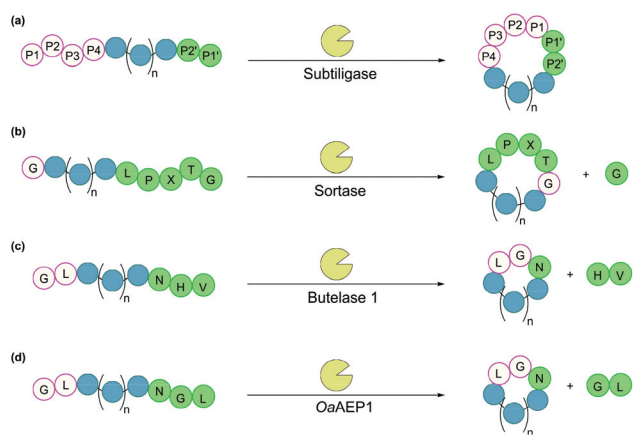
Fig. 6 Enzymatic methods for backbone cyclisation (in some cases recognition sequences may vary): (a) subtiligase, (b) sortase, (c) butelase 1, and (d) OaAEP1.
