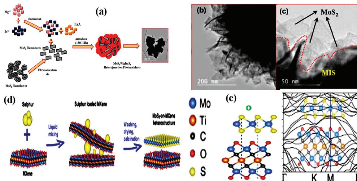
Fig. 6 (a) Schematic diagram showing the growth mechanism and (b) and (c) corresponding HRTEM images of \text{MoS}_2/\text{MgIn}_2\text{S}_4 heterojunction photocatalyst. Reproduced with permission. 90 (d) Schematic representation of the fabrication of \text{MoS}_2/\text{MXene} hybrids and (e) structural stacking patterns and electronic band structure of \text{MoS}_2/\text{Mo}_2\text{TiC}_2\text{O}_2 . Reproduced with permission. 105
