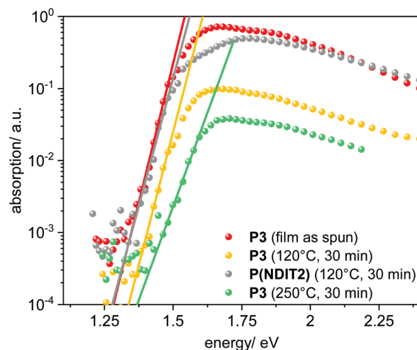
Fig. 6 Comparison between the absorption of P3 ( M_{\text{n}} = 61 \text{ kg mol}^{-1} ) and P(NDIT2) ( M_{\text{n}} = 62 \text{ kg mol}^{-1} ) thin films in dependence of the annealing temperature; measured by photothermal deflection spectroscopy. The solid line displays the corresponding exponential fits for extraction of the Urbach energy U_{\text{E}} . Films were spin-coated (1000 rpm, 60 s) from o -DCB solutions.
