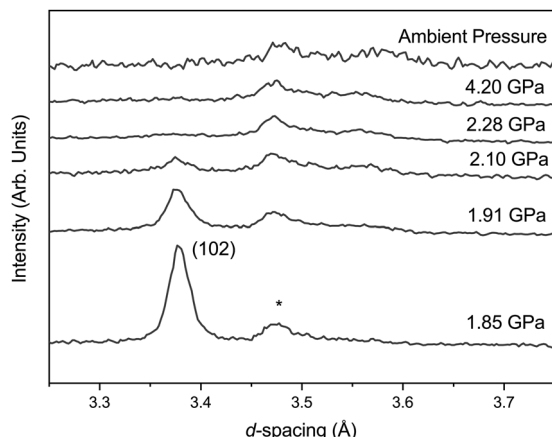
Fig. 2 Neutron diffraction patterns of \text{FePO}_4\text{-I} with increasing pressure. The reflection at \sim 3.37 Å is the (102) reflection of \text{FePO}_4\text{-I} , the reflection at \sim 3.47 Å is the (asterisk) reflection of the \text{Al}_2\text{O}_3 from the anvil and the emerging but broad feature at \sim 3.56 Å can be indexed as the (111) reflection of \text{FePO}_4\text{-II} .
