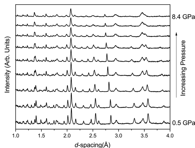
Fig. 3 Neutron diffraction patterns of \text{FePO}_4\text{-II} with increasing pressure.
