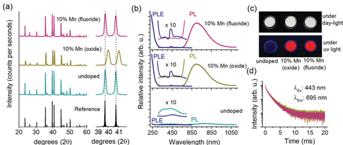
Fig. 2 PXR patterns of undoped and Mn 2+ (10 at%) doped Ca-α-SiAlON obtained using oxide and fluoride doping precursors (a); respective PL–PLE spectra (b); the photographic images (powders filled in quartz disks) under day-light and UV-light (254 nm Hg vapor lamp) exposure (c); and the Mn 2+ PL decay curves (d). The reference XRD pattern in (a) was calculated for Ca-α-SiAlON structure ( \lambda_{K\alpha} = 1.78897 \text{ \AA} ). In (b), the excitation wavelength was 255 nm for PL measurements and the emission was monitored at 695 nm to record the PLE spectra. The insets present enlarged view (10 times) of PL–PLE curves in 300–600 nm range.
