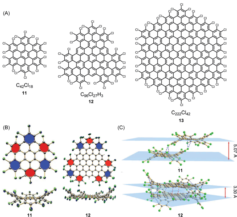
Fig. 1 (A) Examples of chlorinated NGs 11–13 . (B) Crystal structures and (C) crystal packing of chlorinated NGs 11 and 12 . 58 Copyright 2013. Adapted with permission from Macmillan Publishers Ltd: Nature Communications.
