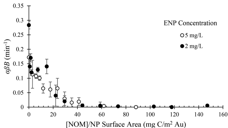
Fig. 4 Pseudo-first order rate constants ( \alpha\beta B ) for attachment of bPEI-AuNPs ( 2\text{ mg L}^{-1} or 5\text{ mg L}^{-1} ) to glass beads ( 20\text{ g L}^{-1} ) in 1\text{ mM} HEPES, 20\text{ mM} NaCl, and varying concentrations of SRNOM. Error bars represent one standard deviation of replicates.
