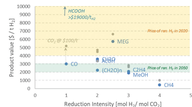
Fig. 7 Affordable price of renewable H 2 for hypothetical CO 2 conversion assuming that the full product value is used to pay for the stoichiometric H 2 consumption, without placeholder for investment and operating costs (cost of renewable H 2 from ref. 60,61; HCOOH: formic acid, MEG: ethylene glycol, CO: carbon monoxide, CH 2 O: formaldehyde, AcOH: acetic acid, C 2 H 4 : ethene, MeOH: methanol, CH 4 : methane, (CH 2 O) n : sugar).
