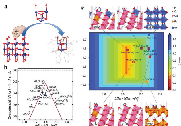
Fig. 16 (a) Structure of \text{Co}_4\text{O}_4\text{-dpk} cubane representing a surface cut-out of the \mu -oxo-bridged \text{CoO}_x catalyst. Reproduced with permission from ref. 26. Copyright 2017, The American Chemical Society. (b) OER volcano plot summarized for a wide range of metal oxide surfaces employing \Delta G_{\text{O}} - \Delta G_{\text{OH}} as a single descriptor. (c) Comparison of the theoretical OER overpotentials on pure \text{WO}_3(001) , \text{CoOOH}(0112) , \text{FeOOH}(010) and Fe,W-doped \text{CoOOH} , where the FeCoW oxyhydroxide shows the lowest overpotential. Reproduced with permission from ref. 315 and 324. Copyright 2017 and 2016, AAAS.
