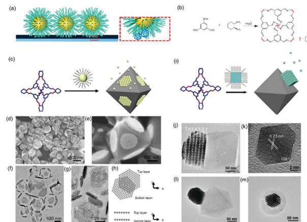
Fig. 7 (a) Schematic illustration of host-guest interaction pairs between nanoparticles and POCs. (b) The chemical reaction of POC synthesis. Schematic illustration of spherical (c) and cubic (i) nanoparticle assembly onto the POC assembled crystals. SEM images (d and e) and TEM images (f and g) of spherical nanoparticle-POC assemblies. (h) The cartoon image of the top and bottom layer of nanoparticles on two facets of POC crystal. (j) TEM image of nanocube-POC assemblies. (k) TEM images of one octahedral nanoparticle. (l and m) TEM images of octahedral nanoparticle-POC assemblies. 63
