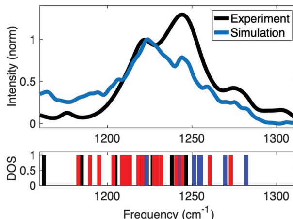
Fig. 10 Comparison of experimental and simulated IR absorption spectrum of \nu_{AS}(\text{PO}_2)^- vibrations and vibrational density of states (DOS) showing the frequency positions of contact pair geometries (blue), solvent separated ion pairs (red) and fully solvated (\text{PO}_2)^- groups (black). Simulations at QM/MM level of theory use a hybrid density functional with exact exchange and empirical dispersion corrections (B3LYP-D, basis: 6-31G* and 6-311+G** for phosphorus atoms) for the QM region and all atoms within 15 Å of the QM region were further included as point charges in the single electron Hamiltonian to account for long-range polarization of the QM region via electrostatic embedding. QM/MM vibrational frequencies were evaluated for all bi-phosphate – tri-ribose segments along the dsRNA helix in double harmonic approximation, followed by averaging over the different spatial positions. Adapted with permission from ref. 85. Copyright 2021 Elsevier.
