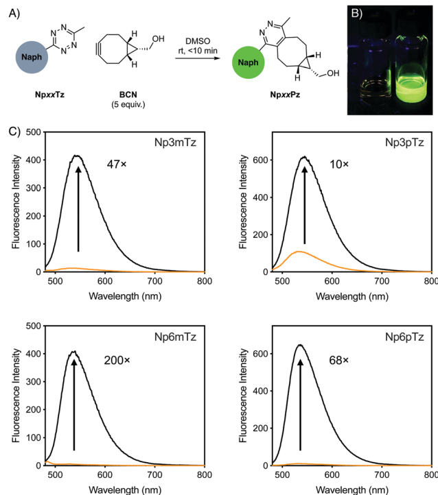
Fig. 2 (A) Schematic of fluorogenic reaction between naphthalimide (Naph) tetrazines after reaction with BCN to form pyridazine products in situ . (B) Photograph of vials of Np6mTz (left) and Np6mPz (right) in dichloromethane, under 365 nm light. (C) Emission spectra of 5 \mu\text{M} solutions of naphthalimide tetrazines (orange) and the corresponding pyridazine products (black). Numbers indicate the fold turn-on as determined by integration of the spectra.
