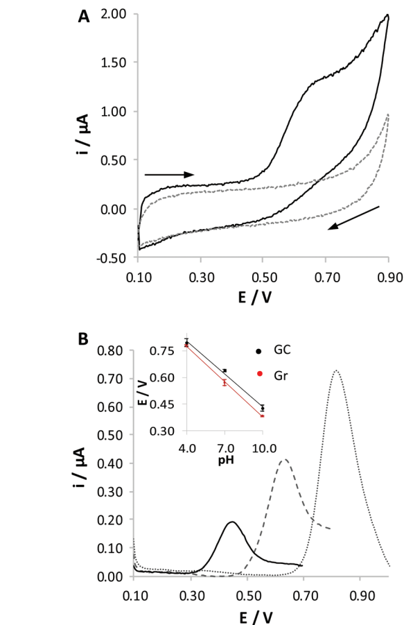
Fig. 1 (A) CV response recorded in the presence (solid line) and in the absence (dashed line) of 0.1\ \text{mM RC} , 0.1\ \text{M BRB} ( \text{pH}\ 7.0 ) at the Gr electrode, 0.050\ \text{V s}^{-1} potential scan rate. (B) DPV responses recorded in similar solutions at the GC electrode, at different pH values: 4.0 (dotted line), 7.0 (dashed line) and 10.0 (solid line), 0.015\ \text{V s}^{-1} potential scan rate; the curves reported are subtracted for the relevant signal recorded in the absence of the analyte.
