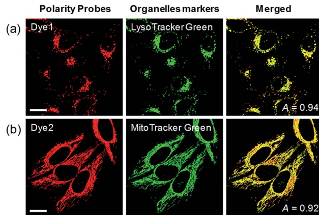
Fig. 3 Co-localization assays in HeLa cells for (a) Dye1 with Lyso-Tracker Green and (b) Dye2 with Mito-Tracker Green, respectively. Excitation wavelengths were 488 nm (organelle markers) and 552 nm (polarity probes) and the corresponding emissions were recorded at 500–540 nm (organelle markers) and 565–650 nm (polarity probes). Scale bars = 20 \mu m.
