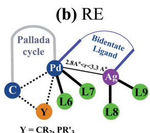
Fig. 2 A generalized representation of (a) concerted metalation–deprotonation (CMD) and (b) reductive elimination (RE) transition states with monometallic and heterobimetallic catalysts. 41 Only the most preferred ligand combinations, obtained by considering a much larger set of possibilities, are shown here. Details of various configurations considered are provided in Section 6 of the ESI. †
