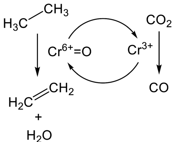
Scheme 1 Redox mechanism for EDH in the presence of CO 2 over Cr oxide catalysts.
