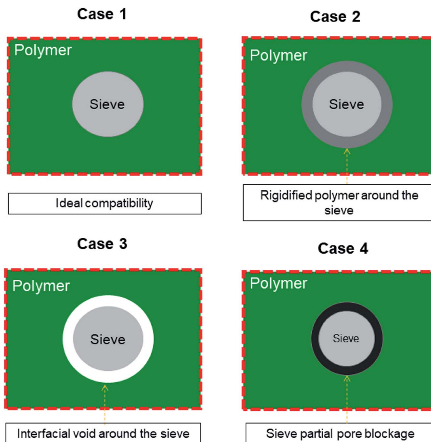
Fig. 1 General representation of different structures at the polymer–filler interface region in MMMs.
