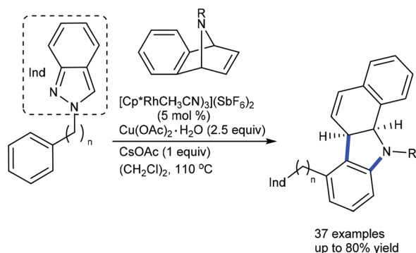
Scheme 132 Coupling of aryl-2 H -indazoles with 7-azabenzonorbomadiene.
