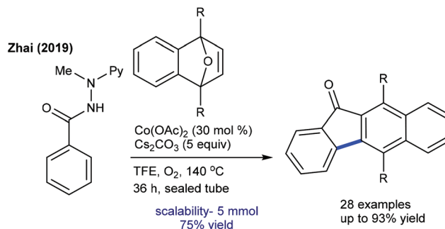
Scheme 131 Synthesis of benzo[b]fluorenones.
