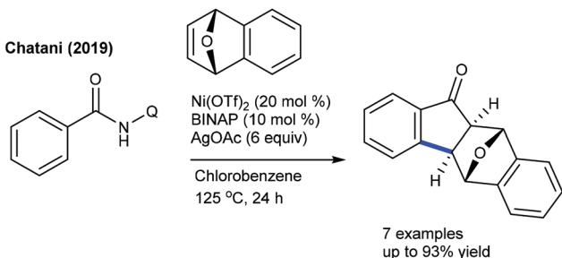
Scheme 130 Reaction of benzamides with oxabenzonorbomadienes.
