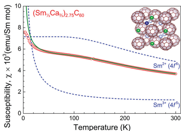
Fig. 1 Temperature dependence of magnetic susceptibilities. Open red circles show the total susceptibility of (\text{Sm}_{1/3}\text{Ca}_{2/3})_{2.75}\text{C}_{60} , obtained after subtracting the diamagnetic core contributions from the difference of the values measured at 4 and 2 T magnetic fields. The calculated magnetic susceptibilities (blue dashed lines) of the free \text{Sm}^{2+} and \text{Sm}^{3+} ions are also included. The susceptibility of \text{Sm}^{2+} ( 4f^6 , ^7F_0 ) is obtained by using van Vleck's formula which takes into account the presence of a J = 1 excited state at 420 K above the J = 0 ground state. For \text{Sm}^{3+} ( 4f^5 , ^6H_{5/2} ), the susceptibility is calculated by considering the sum of the corresponding Curie and van Vleck contributions – in the latter case, the energy difference between the J = 5/2 ground and J = 7/2 excited state is 348 K. The green solid line through the experimental data is the weighted average of the susceptibility calculated assuming 0.68 and 0.32 contributions from \text{Sm}^{2+} and \text{Sm}^{3+} , respectively. The inset shows the building block of the unit cell of the orthorhombic superstructure of the compound, formed by doubling the shown subcell along all three lattice directions. Green and light-grey spheres correspond to off-centred octahedral and tetrahedral (randomly distributed samarium/calcium) metal cations, respectively, while the dark-blue sphere represents the partially-occupied tetrahedral site.
