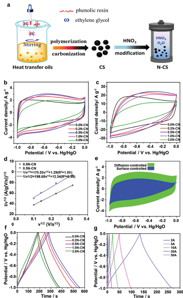
Fig. 14 (a) Schematic illustration of the fabrication of N-doping carbon microspheres from carbon microspheres. CV curves of all the samples at (b) 10 \text{mV s}^{-1} and (c) 100 \text{mV s}^{-1} . (d) Relationship between i(v)/v^{1/2} and v^{1/2} . (e) Surface-controlled (blue) and diffusion-controlled (green) contribution to a current density of 0.5N-CS at 10 \text{mV s}^{-1} . (f) GCD curves of all the samples at 1 \text{A g}^{-1} . (g) Grain size distribution curves of 0.5N-CS from 2 to 50 \text{A g}^{-1} . Reproduced with permission from ref. 99. Copyright 2019 American Chemical Society.
