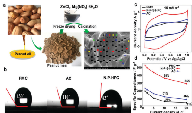
Fig. 26 (a) The preparation process of N-P-S-HPC. (b) Water contact angles of PMC, AC, and N-P-S-HPC. (c) CV curves of PMC, AC, and N-P-S-HPC at 10 mV s -1 in 1 M H 2 SO 4 . (d) Specific capacitances of PMC, AC, and N-P-S-HPC from 1 to 20 A g -1 . Reprinted with permission from ref. 177, Copyright 2019 American Chemical Society.
